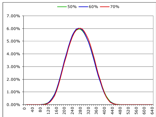
Figure 3. Distribution of a tiebreaker match (5tie) for different values of players winning points on serve.
