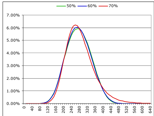
Figure 2. Distribution of an advantage match (4tie1adv) for different values of players winning points on serve.
