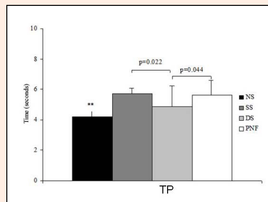
Figure 4. Mean (bars) and SD values of the time (in seconds) taken to reach PP from the beginning of each Wingate Test (WT) trial : WT trials performed after no stretching (NS), static stretching (SS), dynamic stretching (DS), and proprioceptive neuromuscular facilitation (PNF) are presented.
