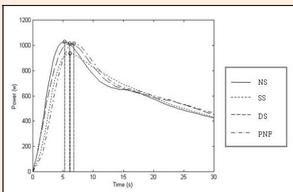
Figure 3. Results of the Wingate Test trials from one participant highlighting instant where the peak power where found (circles), allowing one to observe that stretching tends to delay peak power.
